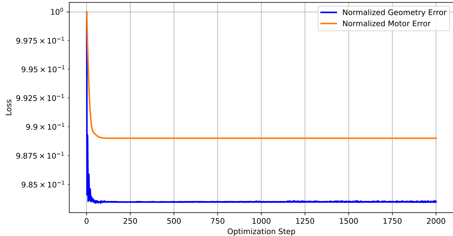
Loss History
